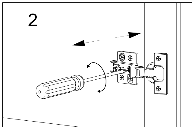
2. Left and Right Adjustment: To shift the cabinet door sideways for alignment.
