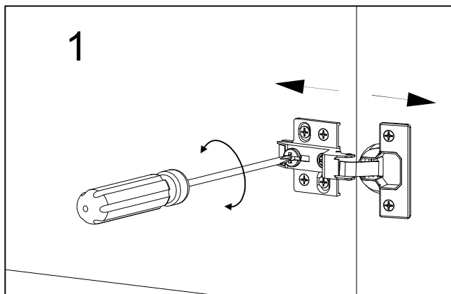
1. Back and Forth Adjustment: To move the cabinet door closer to or farther from the cabinet frame.
