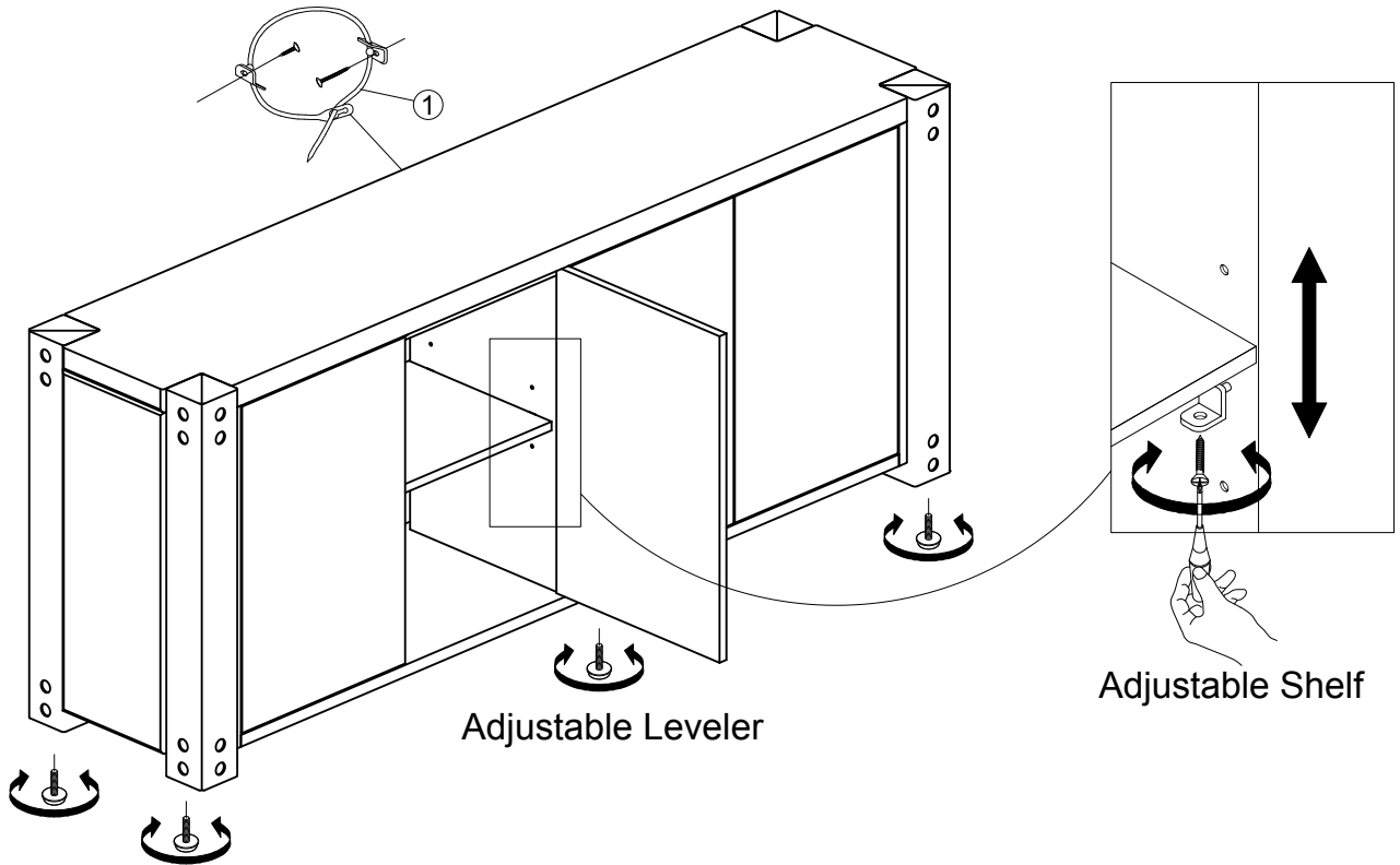
Tipping Hardware
