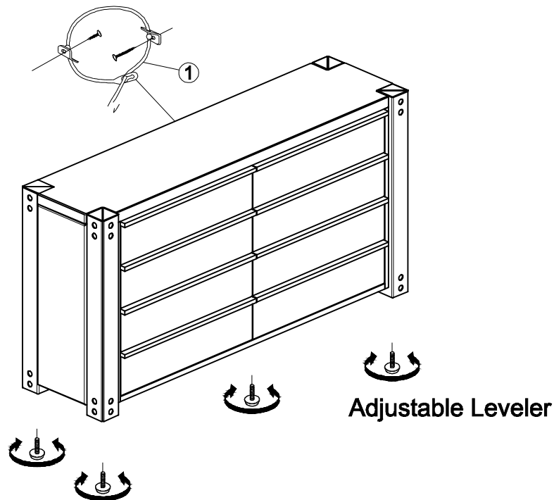
Tipping Hardware
