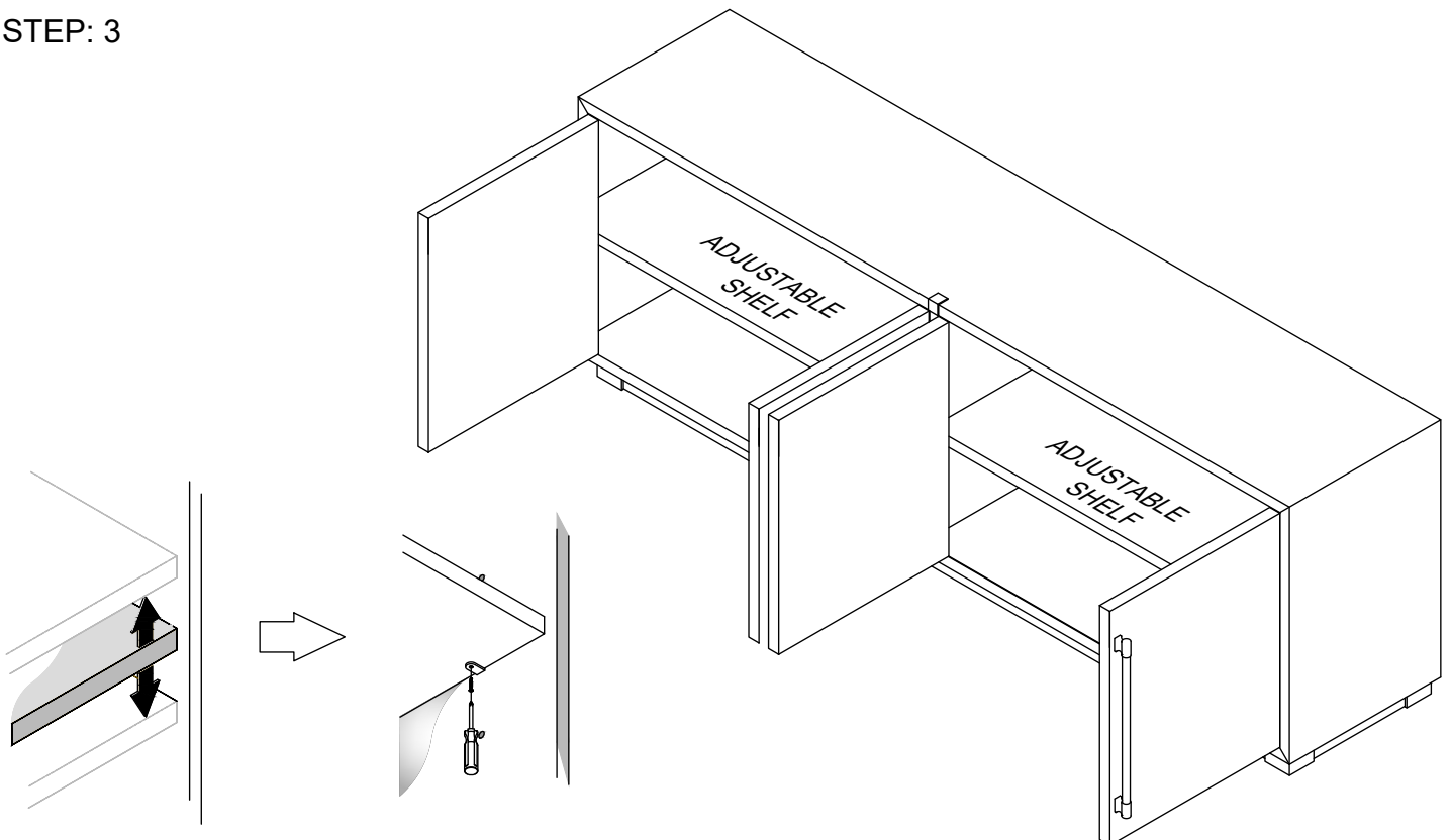
SHELF ADJUSTMENT
