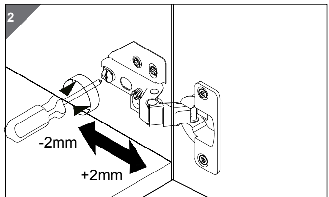
Depth adjustment
