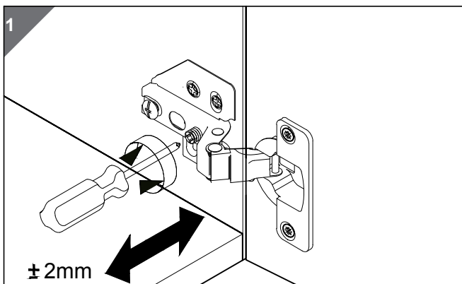
Side adjustment
