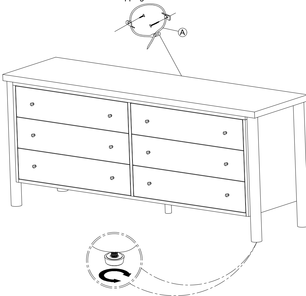
Tipping Hardware
